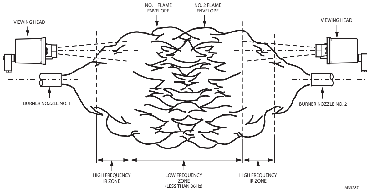
Fig. 8. Sighting opposed fired burners.
