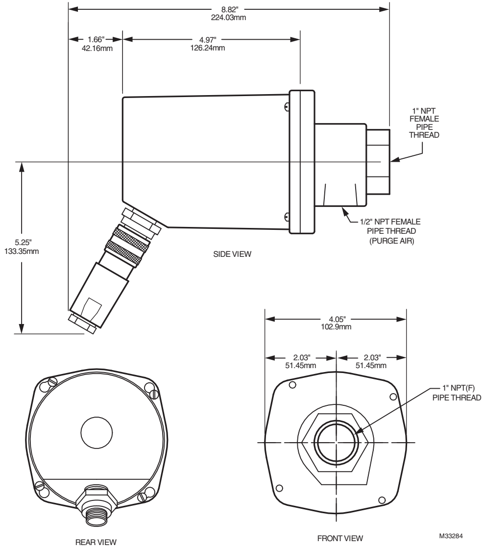
Fig. 2. S550BE, S552BE, and S556BE dimensions in. (mm).
