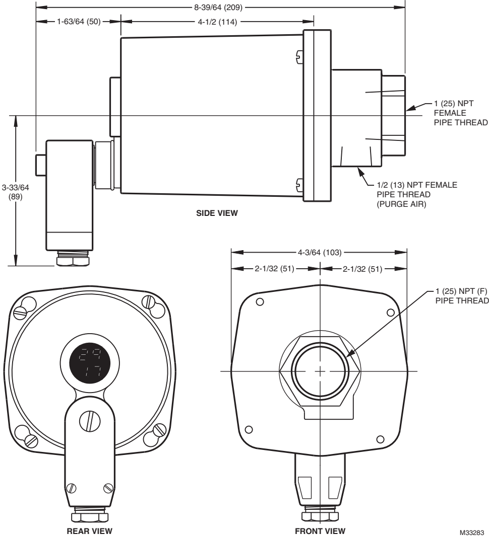
Fig. 1. S550B, S552B and S556B dimensions in. (mm).
