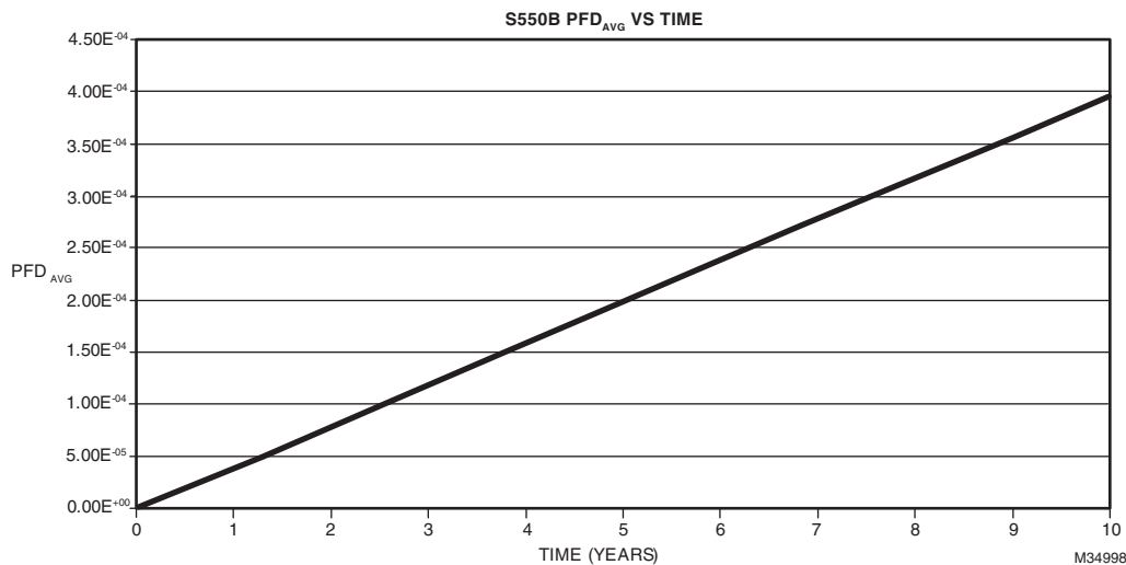
Fig. 11. S550B PFD AVG vs Time.
